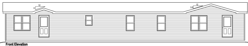
Front Elevation
